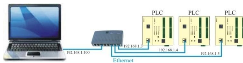
Figure (6.6): PLC Ethernet connection
