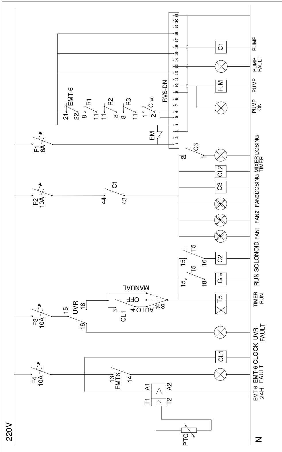
Figure (3.3): Control circuit diagram 220V AC
